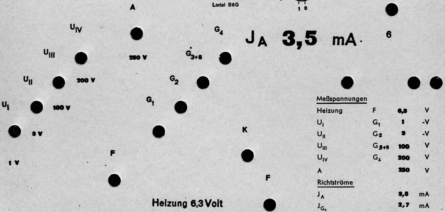
Loctal B8G
